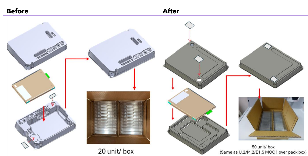
Figure 1. Before and after comparison of the E3.S 7.5mm MOQ1 clamshell packaging redesign. The redesigned clamshell incorporates updated packaging features and increases packaging density
